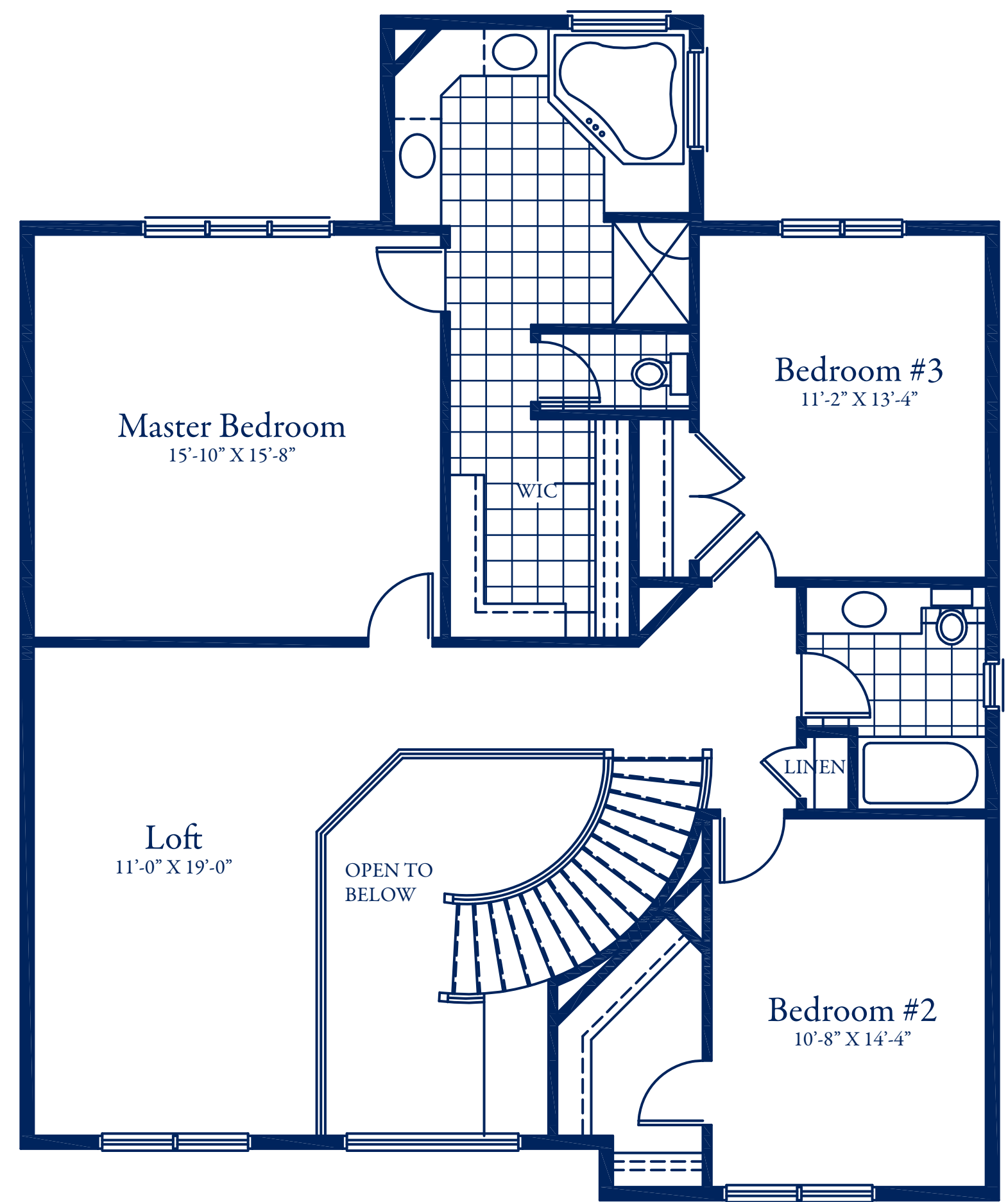
SECOND FLOOR 1336 Sq. Ft.
